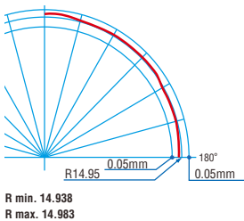
SWB-HM-H type Insert for Semi-finishing
