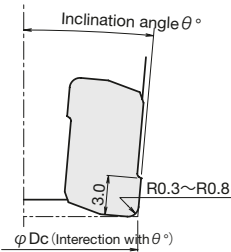
Fig.2 YPHW Type
