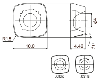
Fig.1 SPNW100415ZTR
