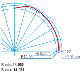
SWB-HM type for Regular purpose insert
