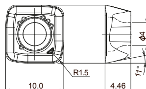
Fig.3 SPMT100415ZPER-SM
