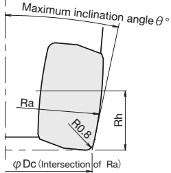
Fig.1 XPHW/T Type
