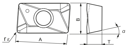
Fig.2 Peripheral Insert
