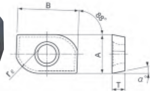
Fig.5 Bottom side insert
