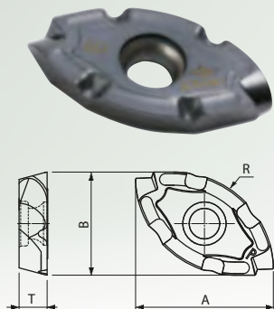
Fig.1 (Main blade for low cutting forces)
