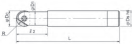
Fig.1 (Straight Neck)
