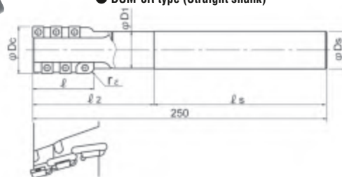
● DUM-6R type (Straight shank)
