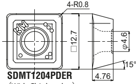
SDMT1204PDER (With Chipbreaker) (Grade : JC605W)
