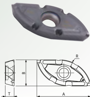
Fig.2 (Sub blade for low cutting forces)
