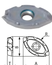
Fig.5 (Main blade)
