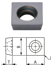
Fig.10 (Peripheral blade)
