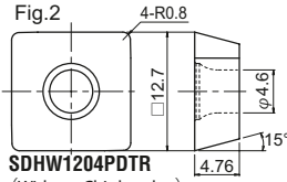
SDHW1204PDTR (Without Chipbreaker) (Grade : JC8015)
