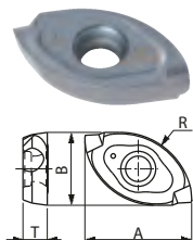
Fig.4 (Main blade)
