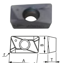
Fig.12 (Peripheral blade)
