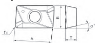
Fig.5 Bottom side insert
