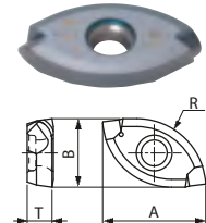
Fig.12 (Peripheral blade)
