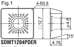
SDMT1204PDER (With Chipbreaker) (Grade : JC8050, JC5040)
