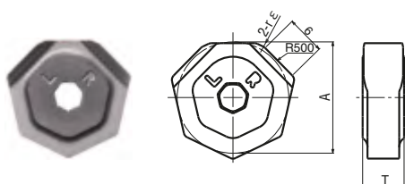
Fig. 3 (Wiper insert)
