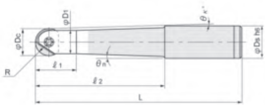
Fig.2 (Taper Neck)
