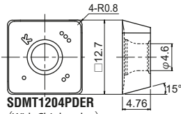
SDMT1204PDER (With Chipbreaker) (Grade : JC8015)
