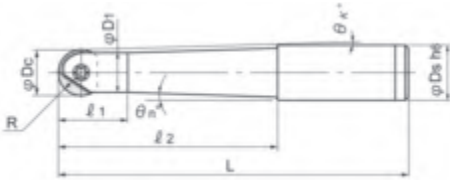
Fig.2 (Taper Neck)
