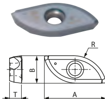
Fig.9 (Sub blade for welded &amp; hardened steel)
