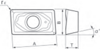
Fig.4 Shank side insert
