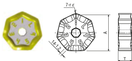
Fig. 3 (Wiper insert)
