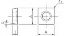
Fig.3 Bottom side insert
