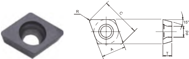
XDHW TYPE
