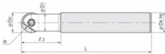
Fig.1 (Straight Neck)
