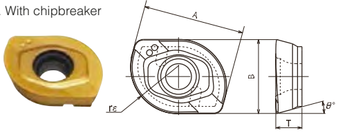
● Fig 2. With chipbreaker
