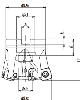
Fig.1 Through Coolant Hole
